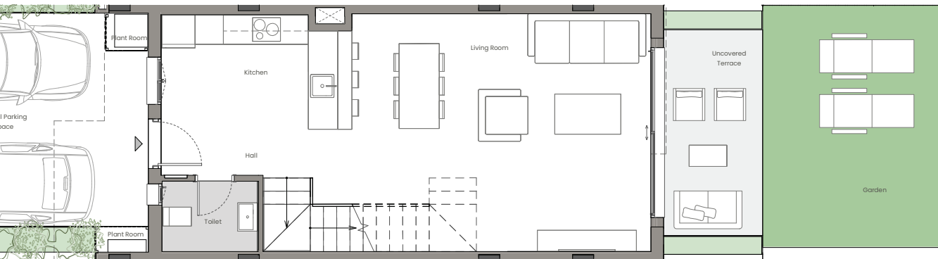
GROUND FLOOR
